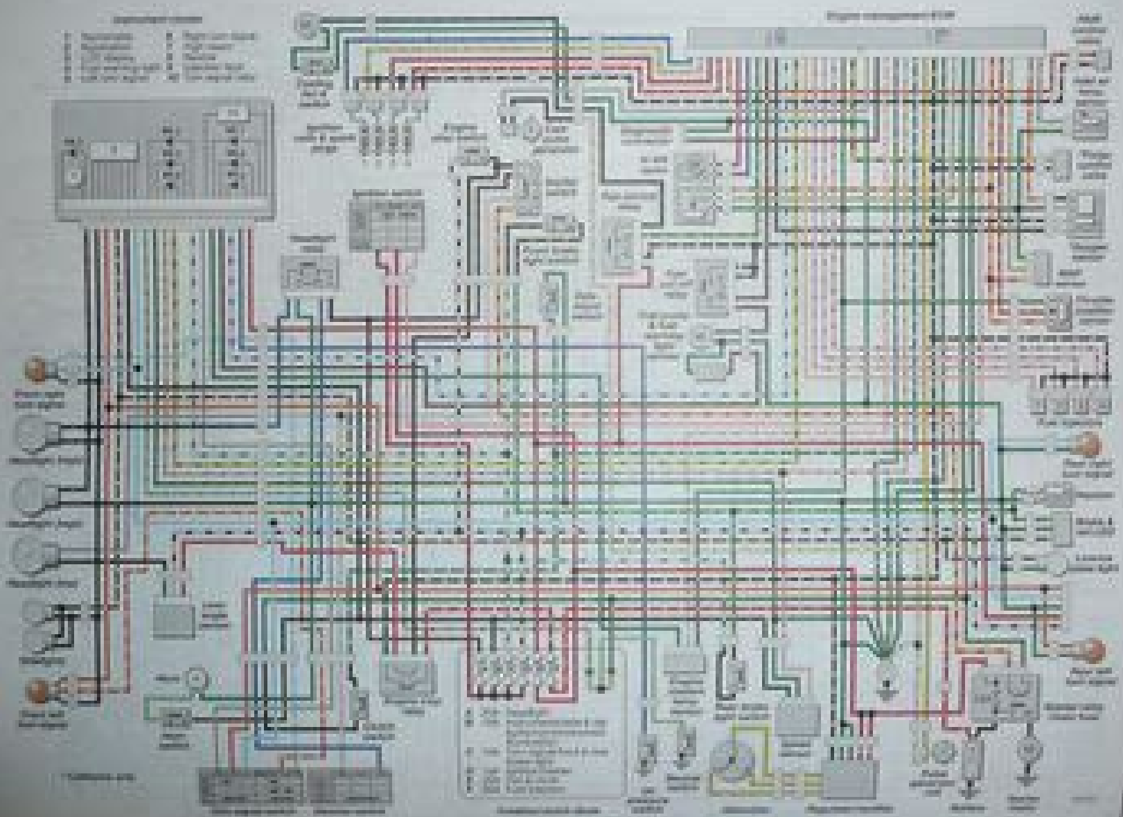
FIGURE 9-22 WIRING DIAGRAM OF A VEHICLE
