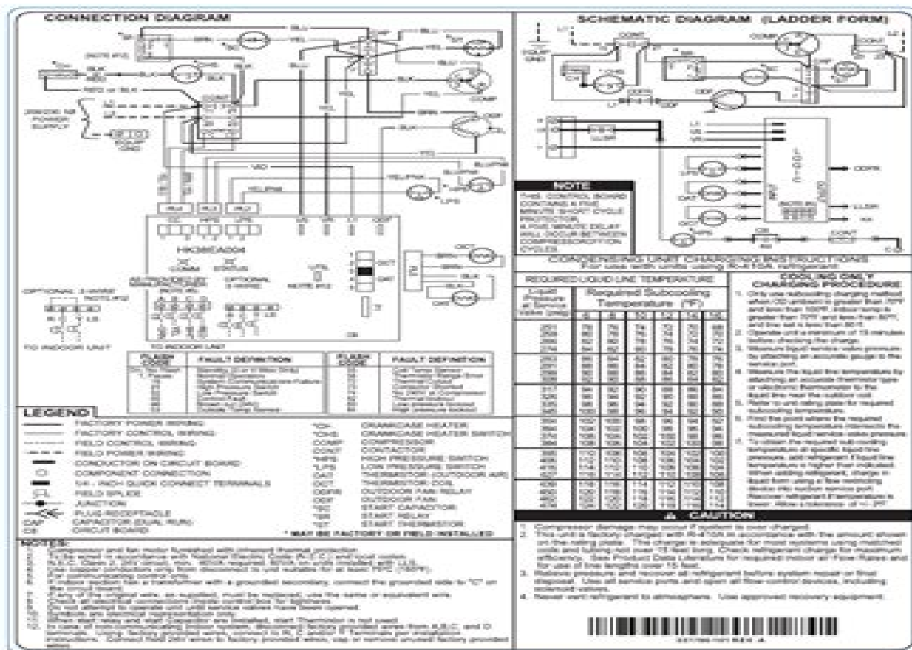
Fig. 1 — Wiring Diagram — 185EN/018, 24, 36, 42, 48 and 600, 208/230-1
