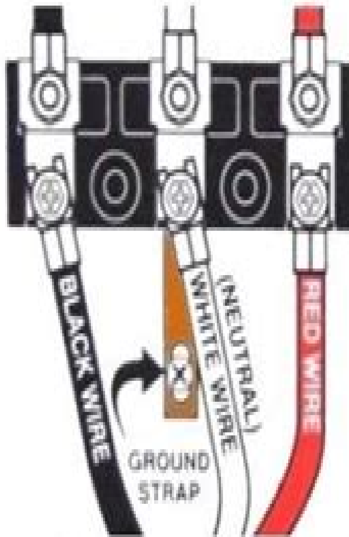
Figure 6- Connecting the wires
