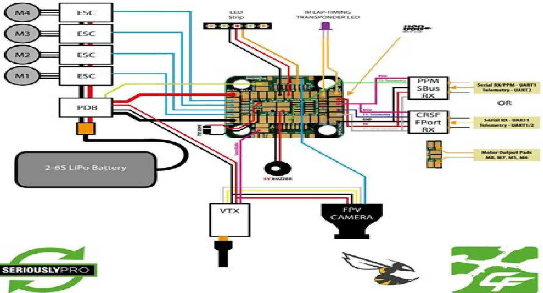
Connection Diagram for FPV Quadcopter for NANO-S version using separate ESCs
