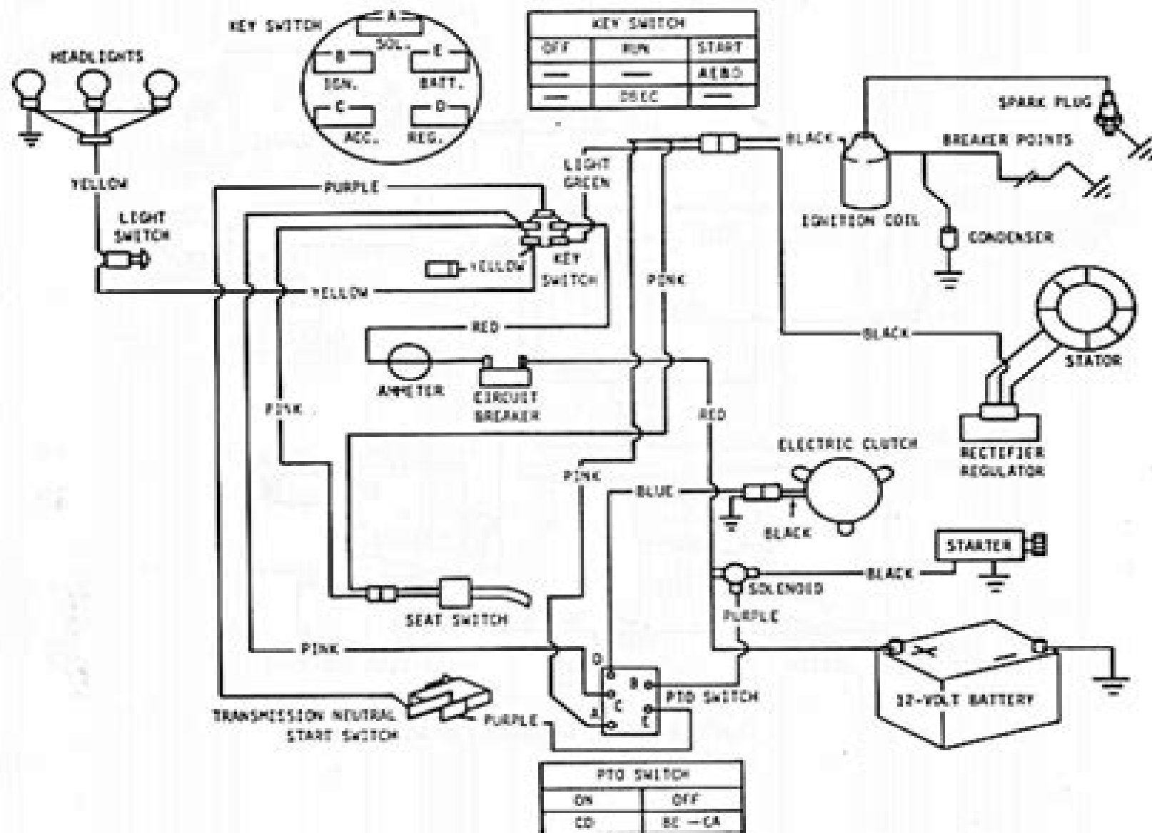
Fig. 4-Wiring Diagram For 210, 212, 214 and 216 Tractors (Serial No. 190,001- )
