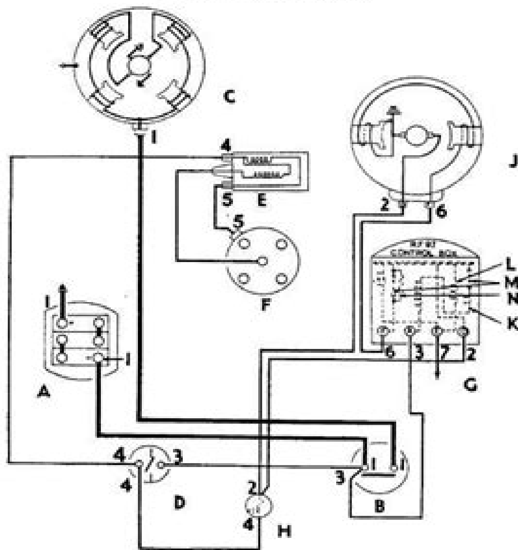
TRACTOR WIRING DIAGRAM.
