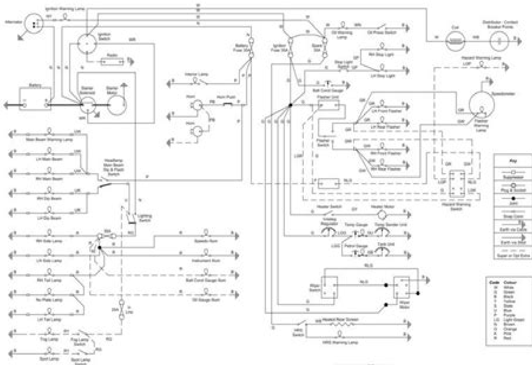
Robin Wiring Diagram - Draft
