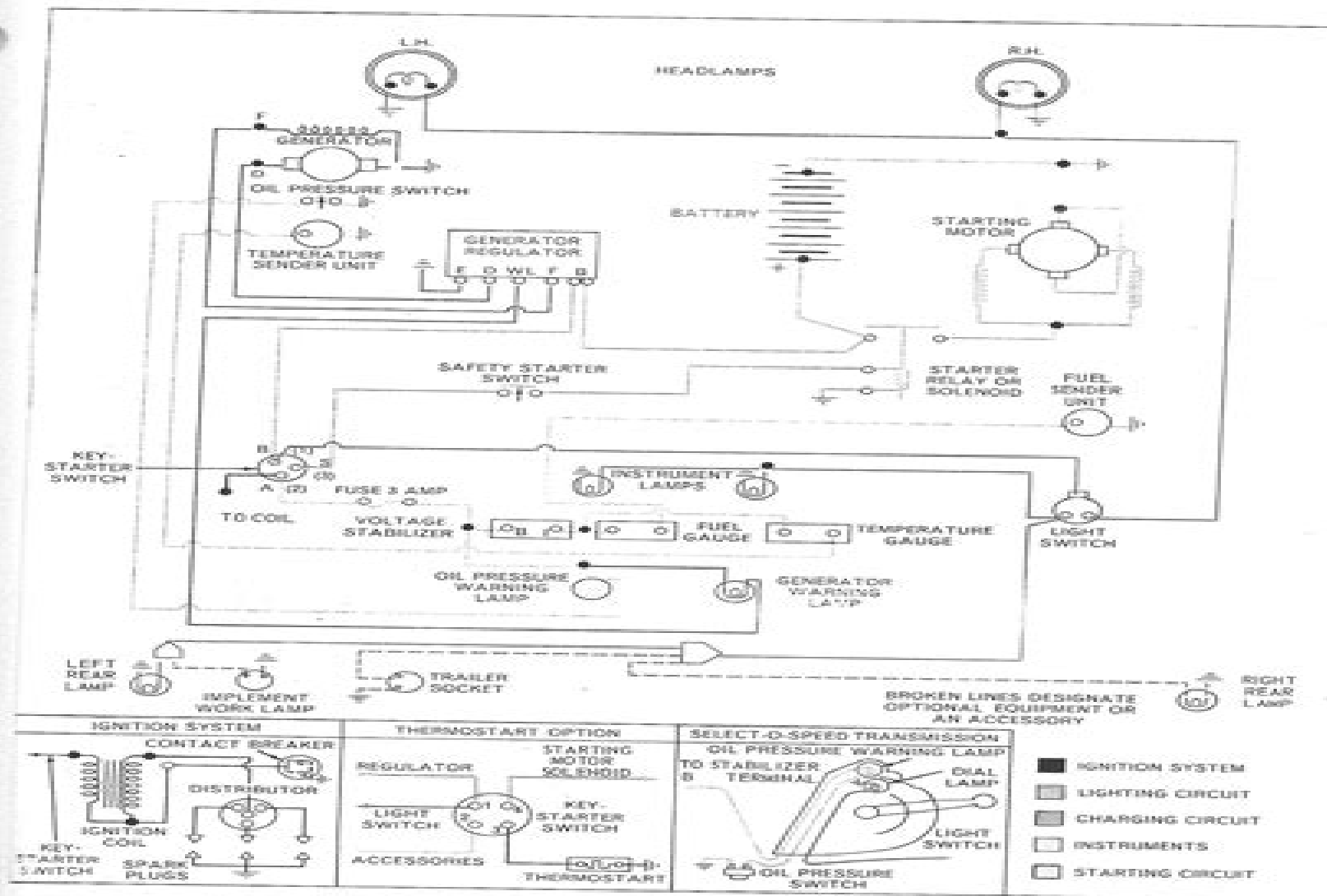
Figure 3 Electrical System Schematic—Tractors with "C" Prefixed Serial Numbers
