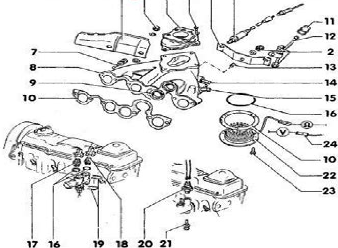
1.0b Mono-Jetronic system inlet manifold and associated components
