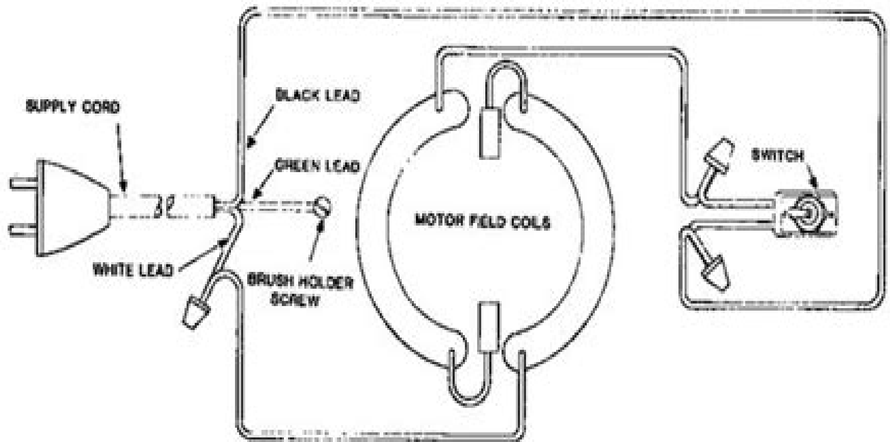
WIRING DIAGRAM 33595
