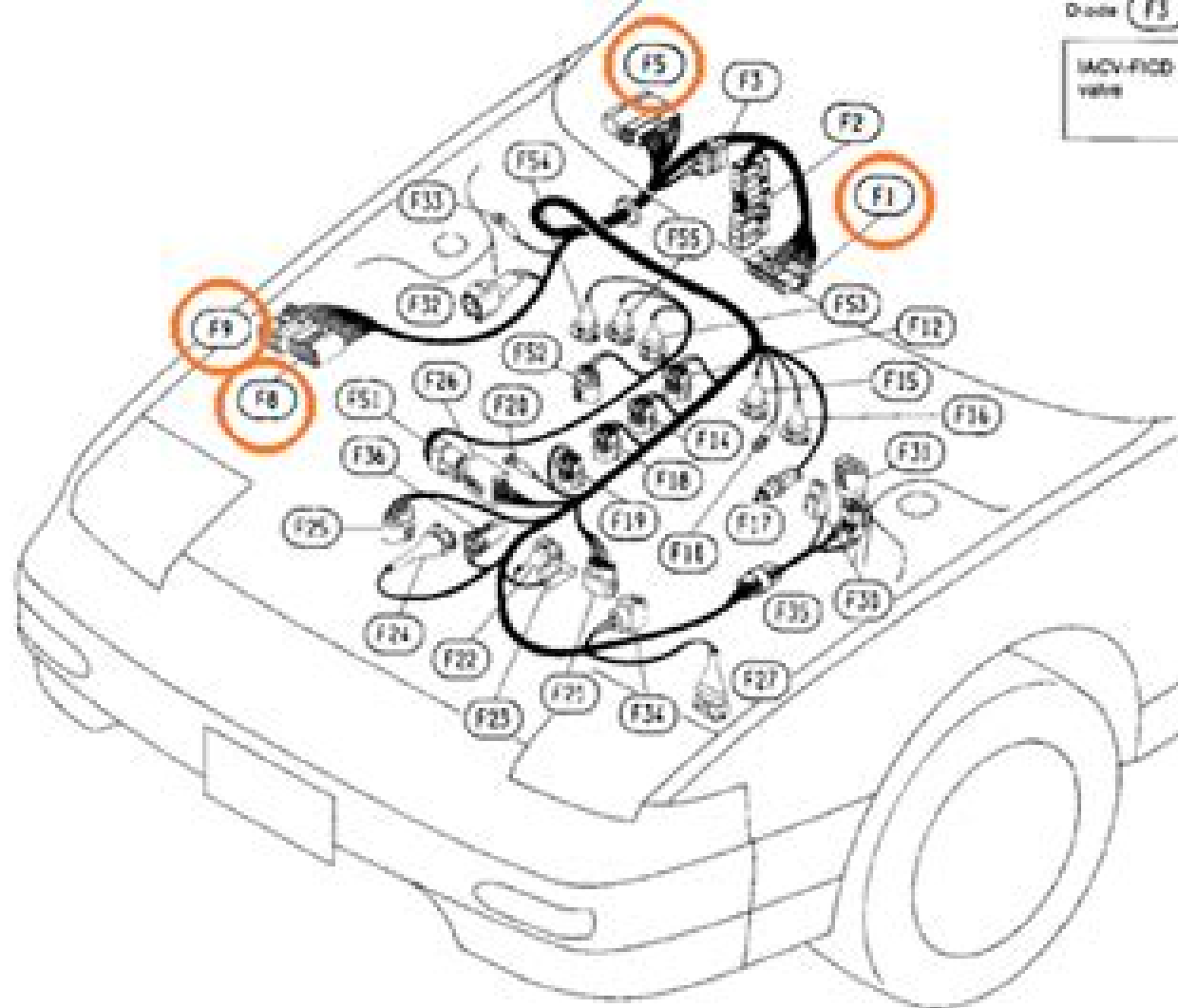
Diode (F3)
