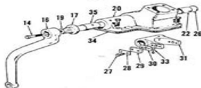
Fig. 17—Exploded view of Model 885 and 885M steering gear housing, cross shaft and steering (drop) arm. Spline (30) are provided to adjust ball nut peg (29) preload against ball nut.
