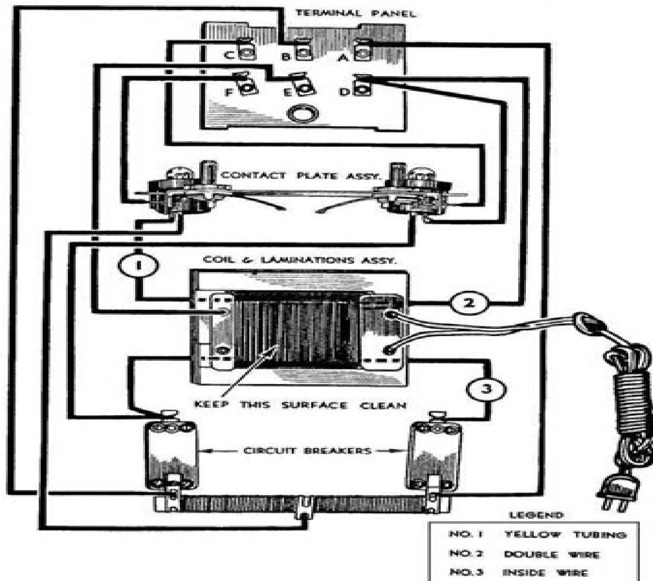
TYPE "R" TRANSFORMER PICTORIAL WIRING DIAGRAM
