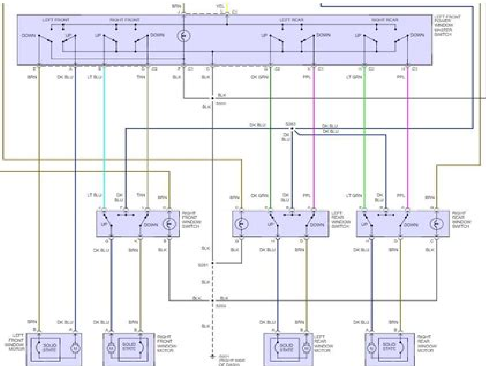
Fig 2: Power Window Circuit, 4 Door
