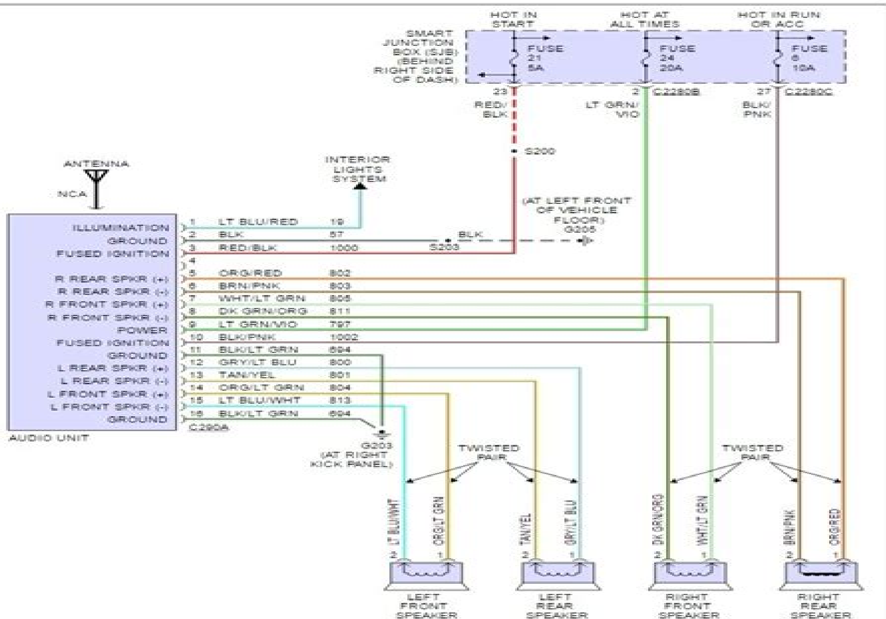
Fig 2: Base Radio Circuit, W/O Audiophile System
