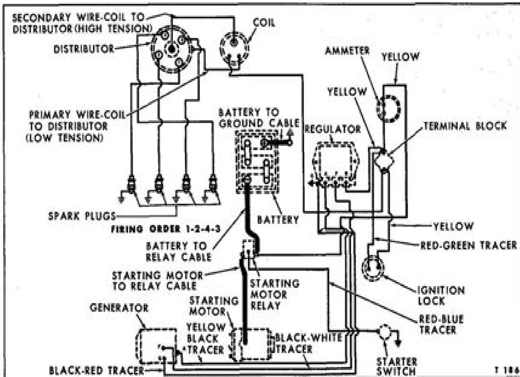
Figure 1—Electrical System Wiring Diagram 6—Volt
