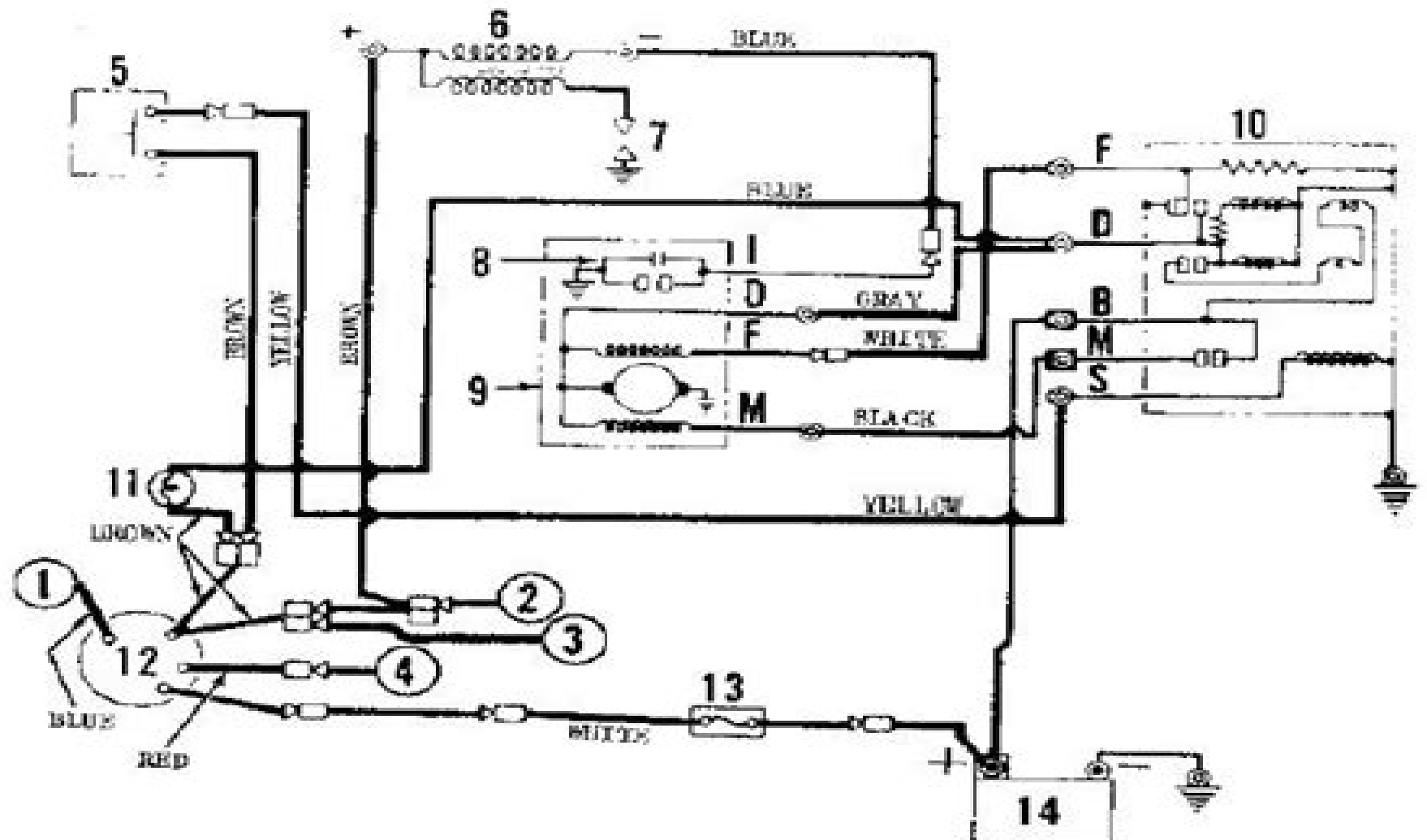
Fig. K2-5—Diagram of ignition, generator and starter systems typical of F1, F1TR, F2, F2TR and F3 models.
