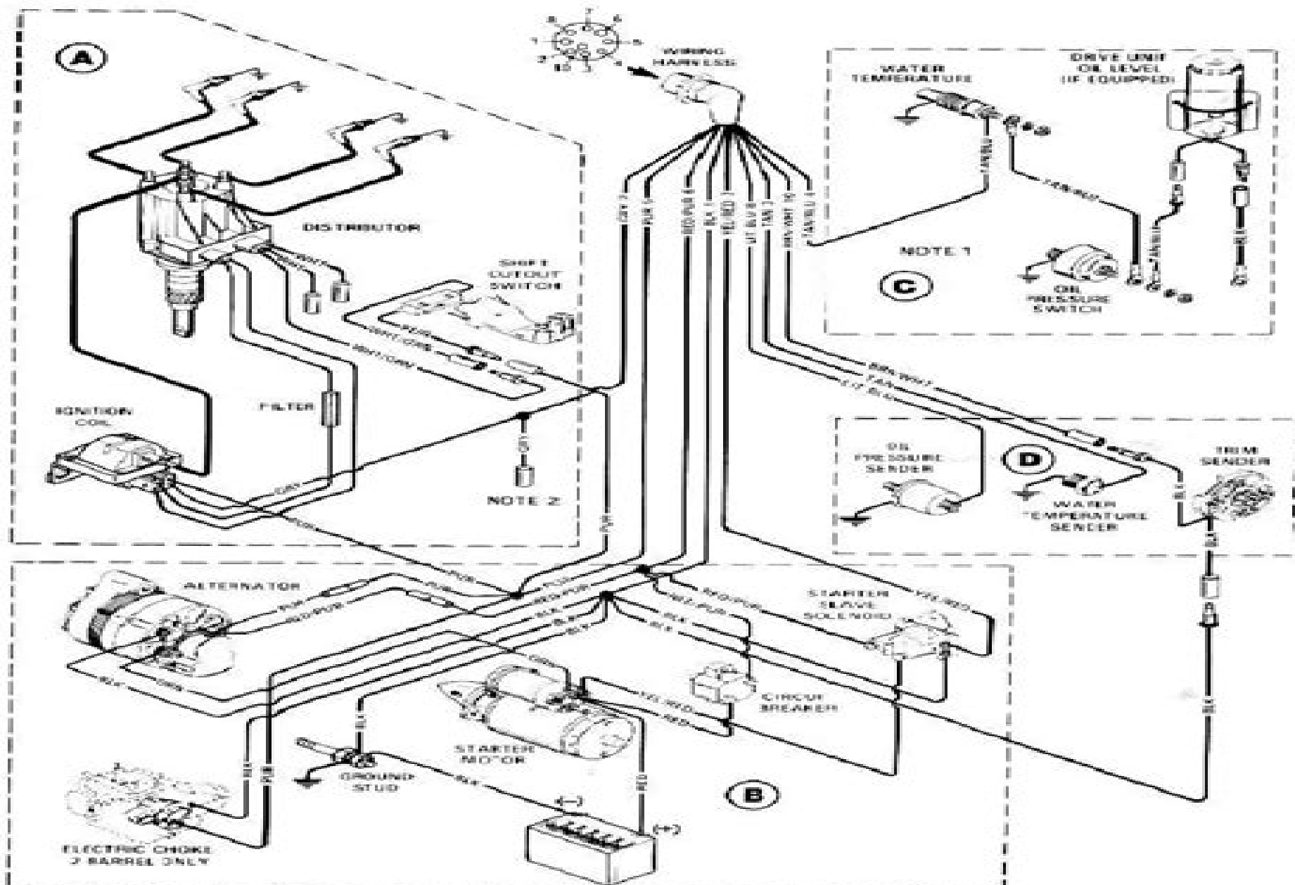
A: Ignition and Choke System B: Starting and Charging System
