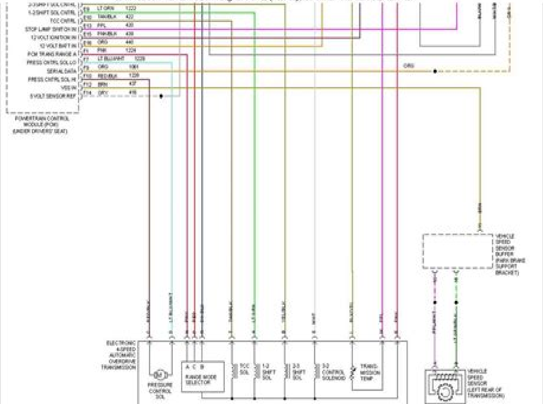
1993 GMC Vandura G2500 Fig. 1: 5.7L (VIN K), Transmission Circuit, 4L60-E
