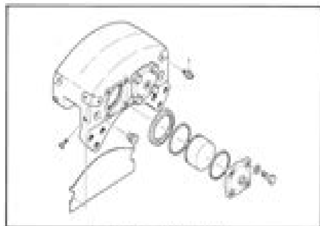
Fig. 13. Bleed Brake Head (Exploded View)
