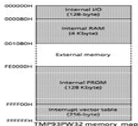
TMP93PW32 memory map
