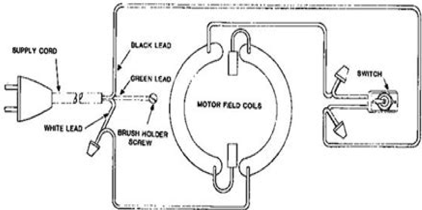
WIRING DIAGRAM 33595
