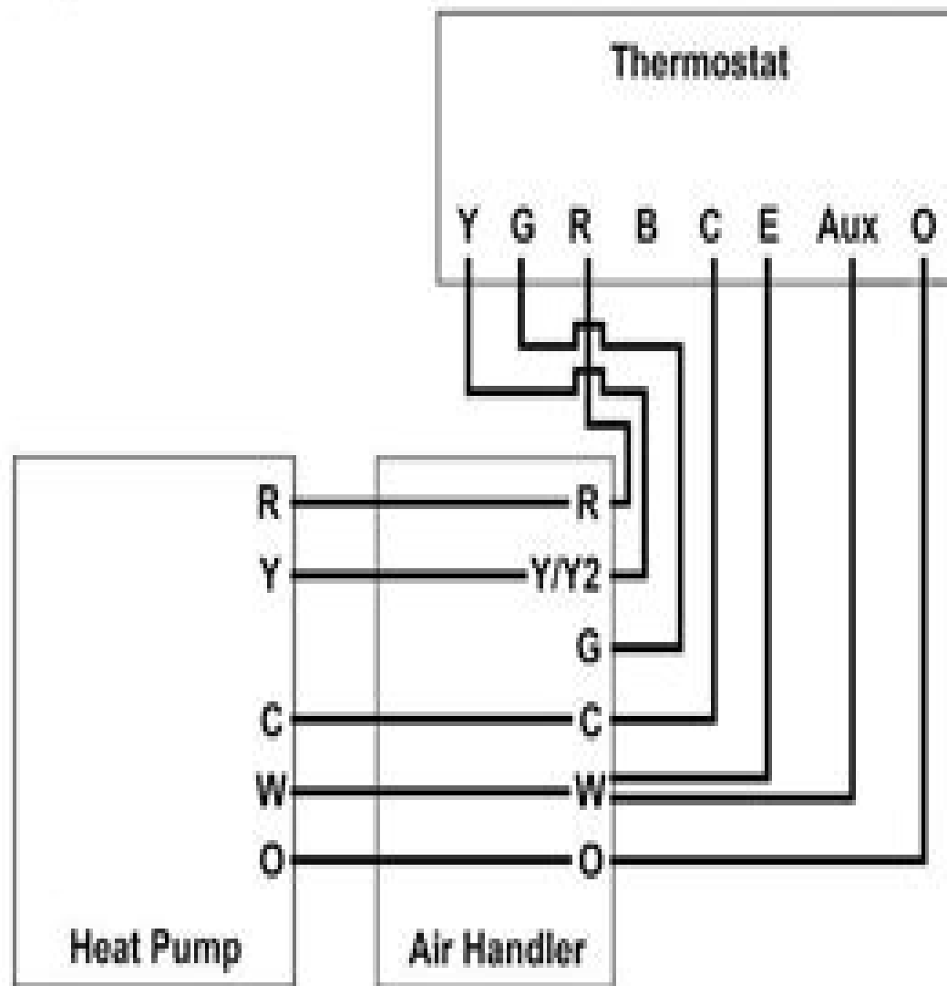
Wiring Diagram for Air Handler with Electric Resistance Heat and Heat Pump
