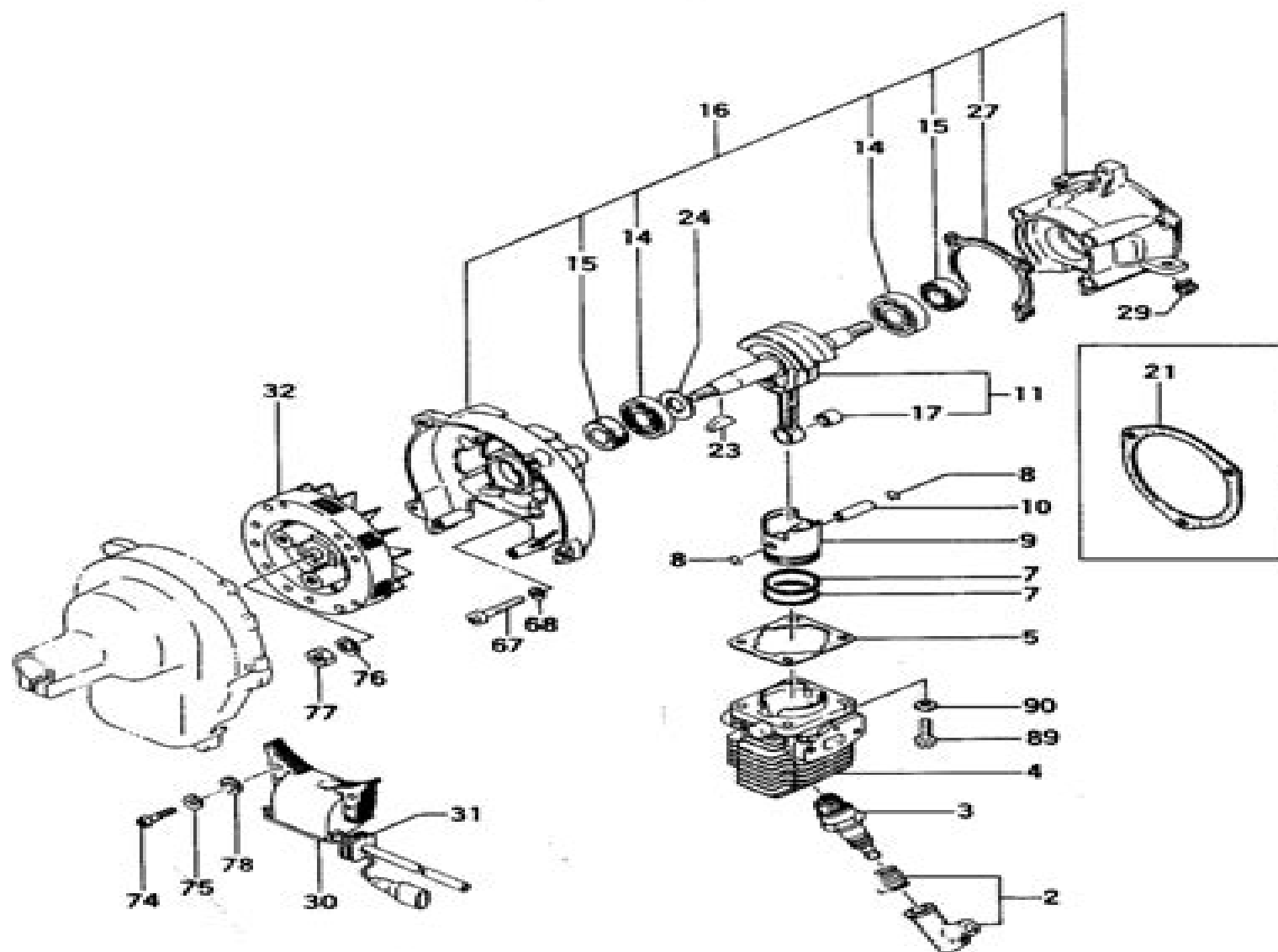
FIG. 1 ENGINE
