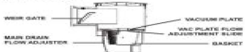
* Figure 2: XP5000 Skimmer Box (side view)
