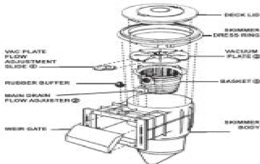
* Figure 1: SP5000 Skimmer Box
