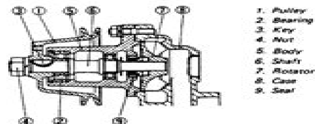
Fig. 39. Water Pump
