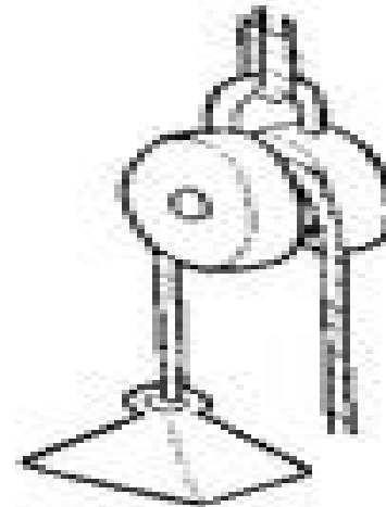
PULLEY
