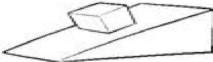
INCLINED PLANE
