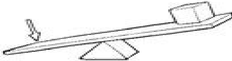
LEVER
