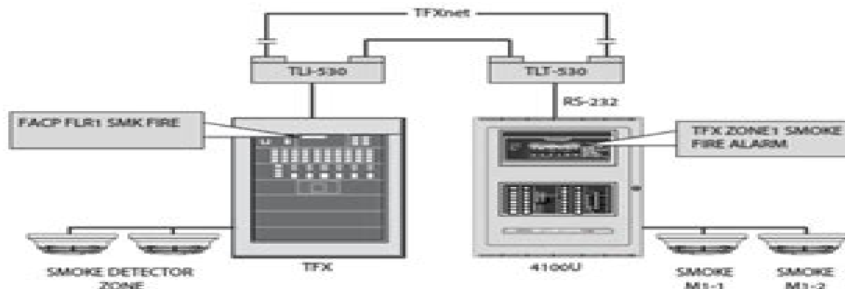
Figure 1 TF30 Functional Overview (4100U Shown)
