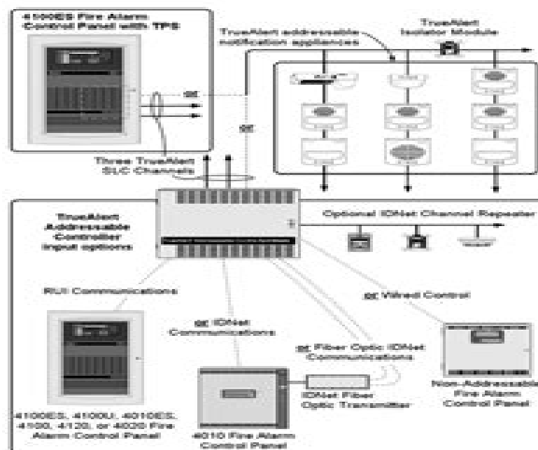
TrueAlert Addressable Operation Reference Diagram
