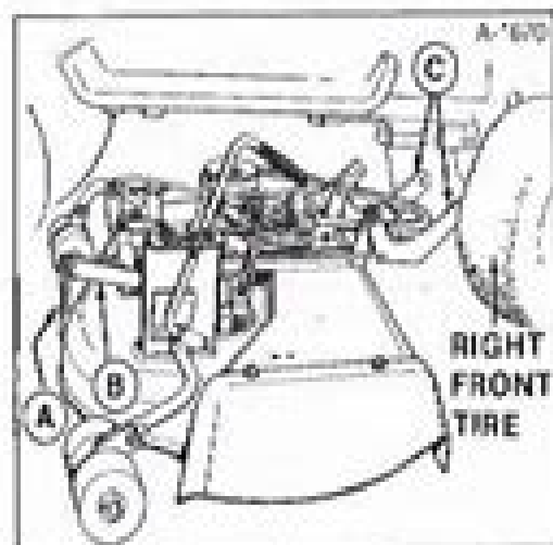
Figure 1. Installing 35" Mower
