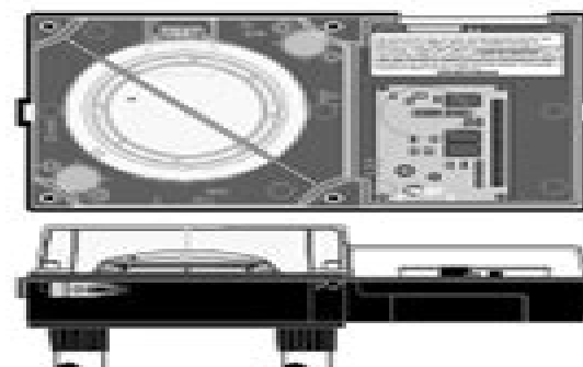
Duct Detector Housing, Front and Bottom View
