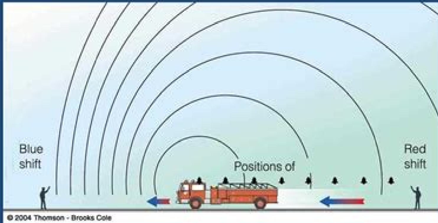
Figure 6.11: The Doppler effect. (b) The clanging bell on a moving fire truck produces sounds that move outward (black circles). An observer ahead of the truck hears the clangs closer together, while an observer behind the truck hears them farther apart.
