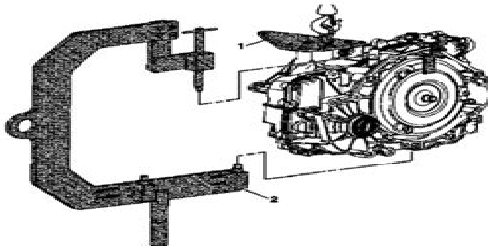
Fig. 1: Identifying Lift Plate & Holding Fixture Courtesy of GENERAL MOTORS COMPANY
