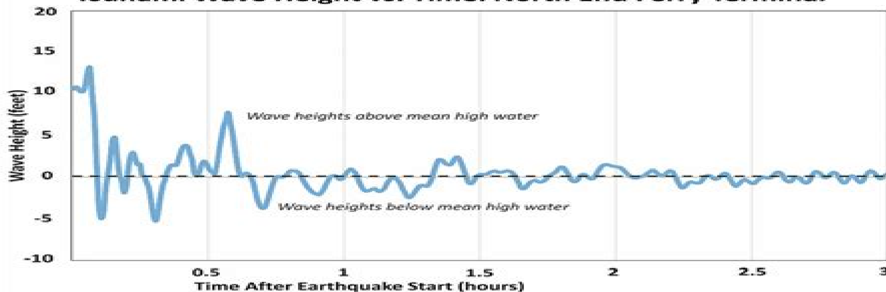
Tsunami Wave Height vs. Time: North End Ferry Terminal
