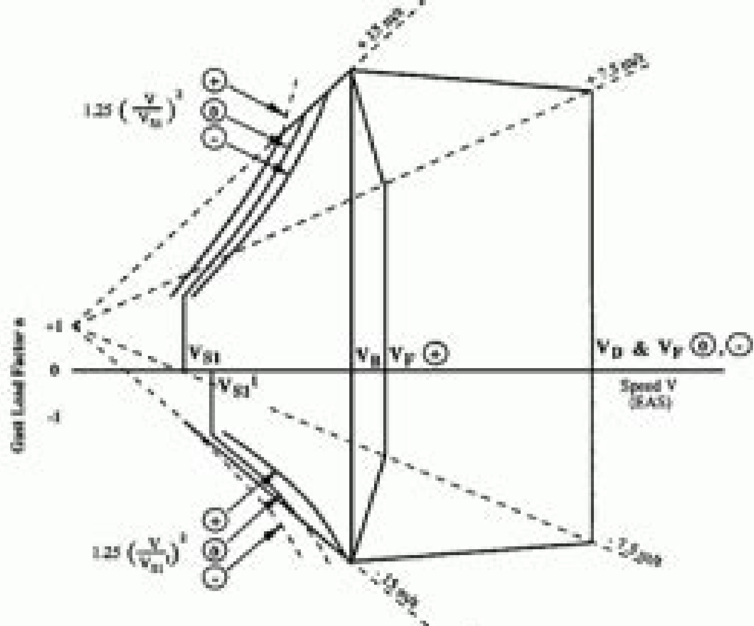
FIGURE 1 GUST ENVELOPE
