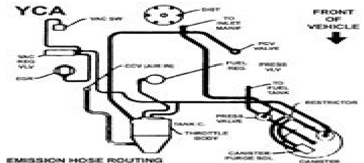
1986-1989 2.8L FUEL INJECTED
