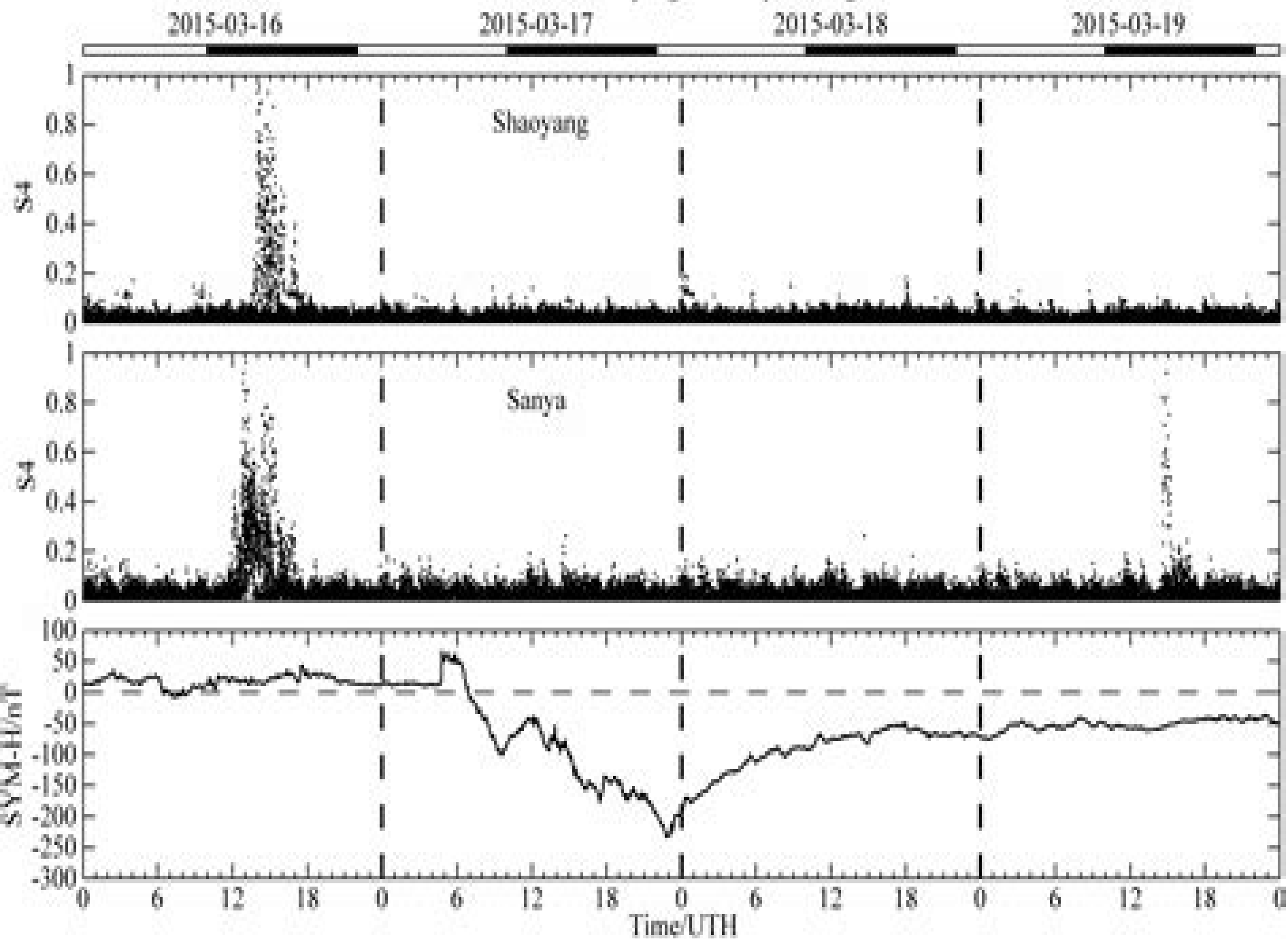
S4 values observed over Shaoyang and Sanya during 2015-03-16—19
