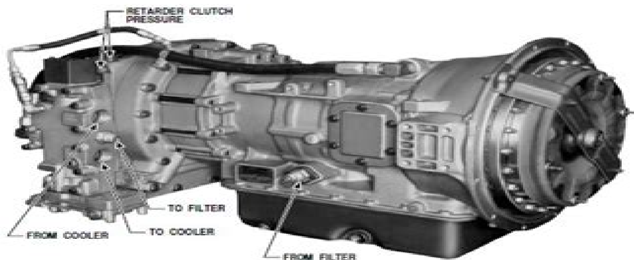
Figure 3-16. MTB Retarder Check Points — External Connections, Right-Front View
