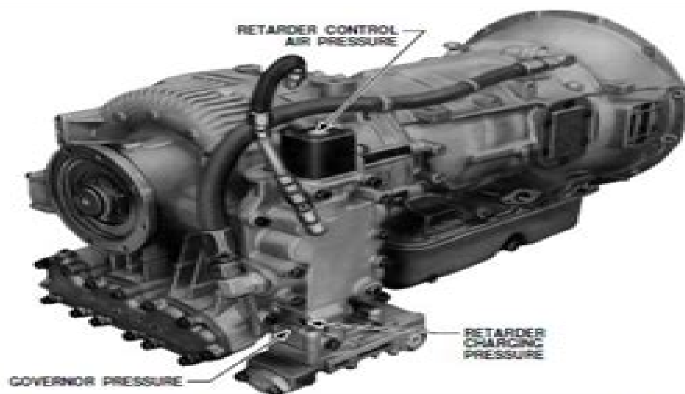
Figure 3-17. MTB Retarder Check Points — External Connections, Right-Rear View
