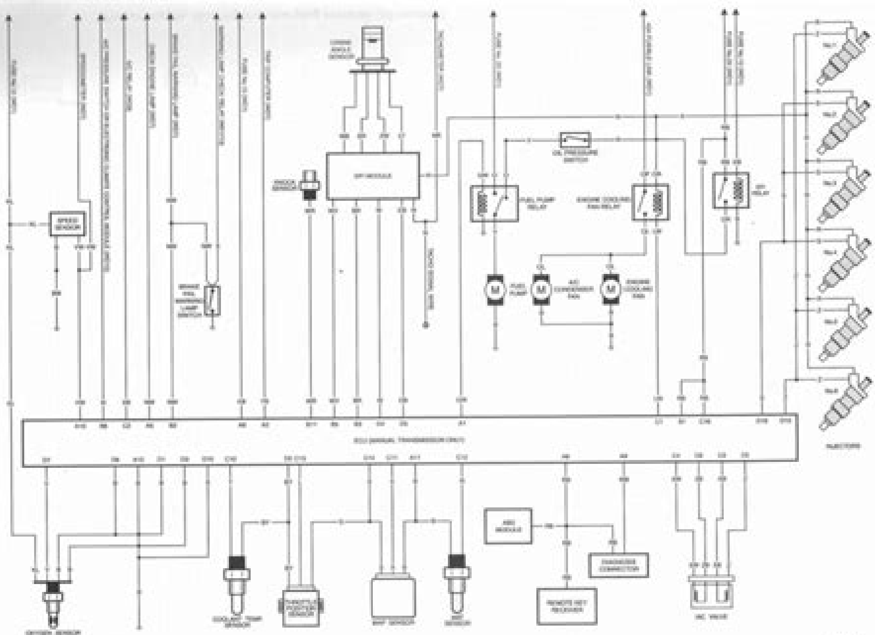
Fuel and engine management system (manual transmission models).
