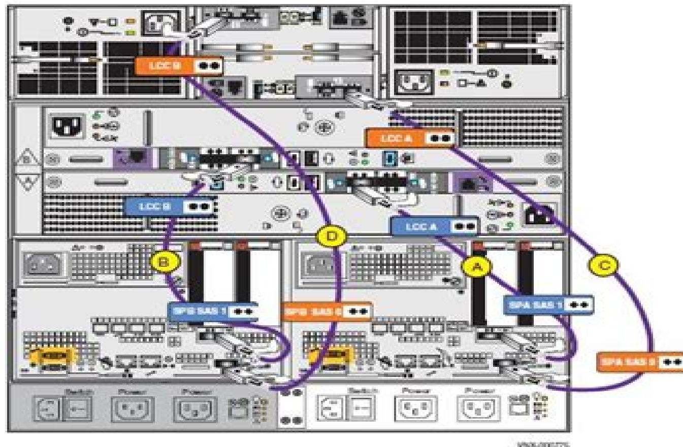
Figure 20 Cabling the first two DAEs to the storage processors
