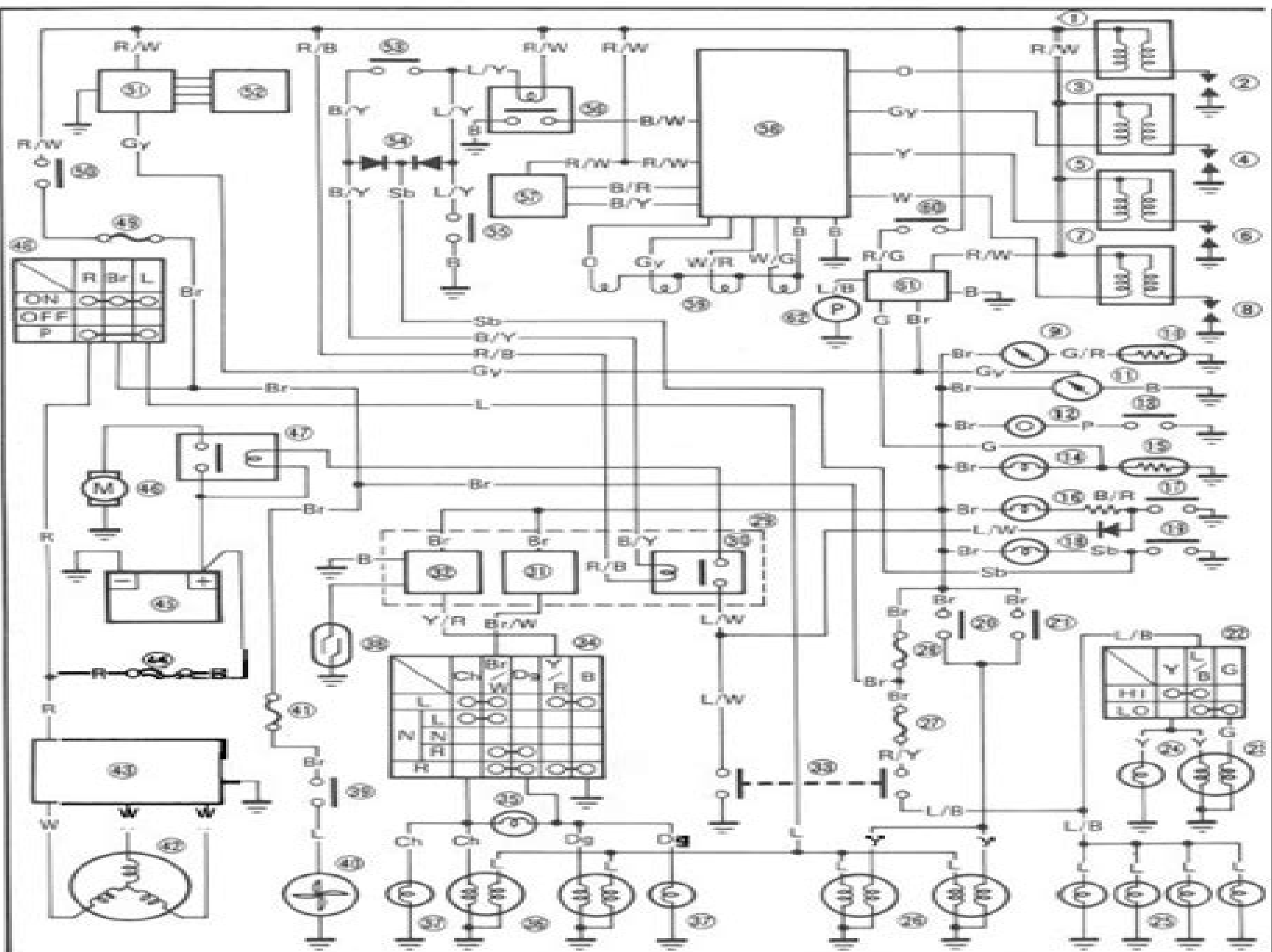
VMX12N/NC CIRCUIT DIAGRAM
