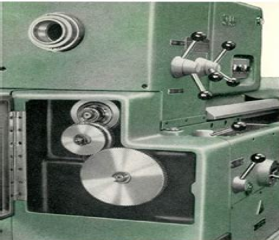
Change gears
