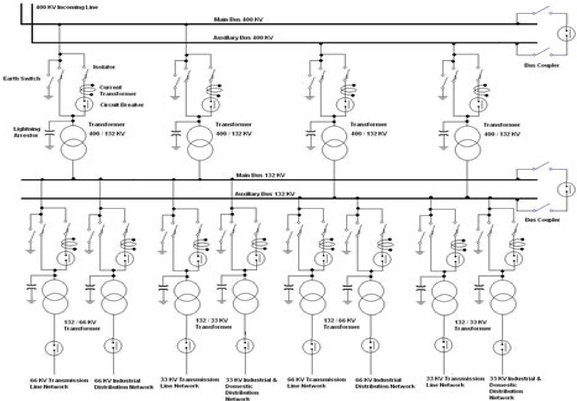
400 / 132 / 66 / 33 kV Outdoor Substation Layout
