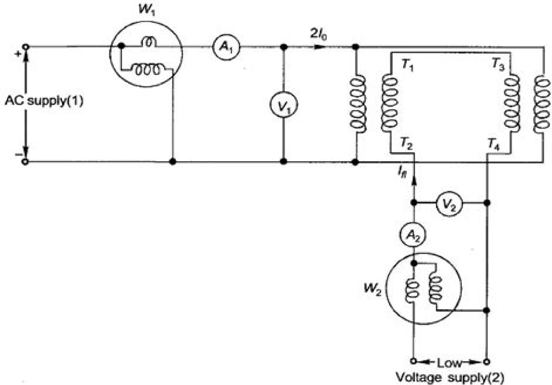
Fig. 3.25 Sumpner's test on two identical single-phase transformers
