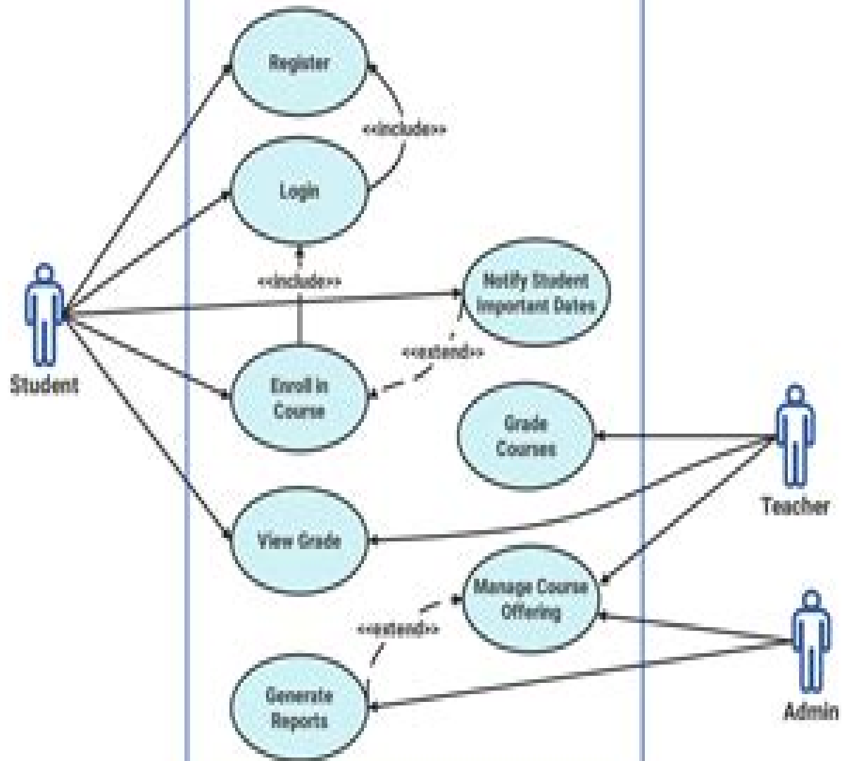
Use case diagram for university management system
