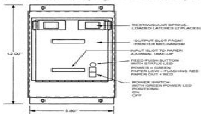
Figure 1: Panel-Mounted Printer, Front View
