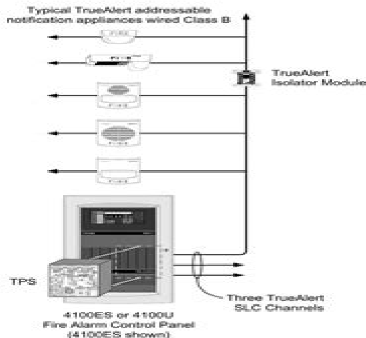
TrueAlert Power Supply Reference Drawing
