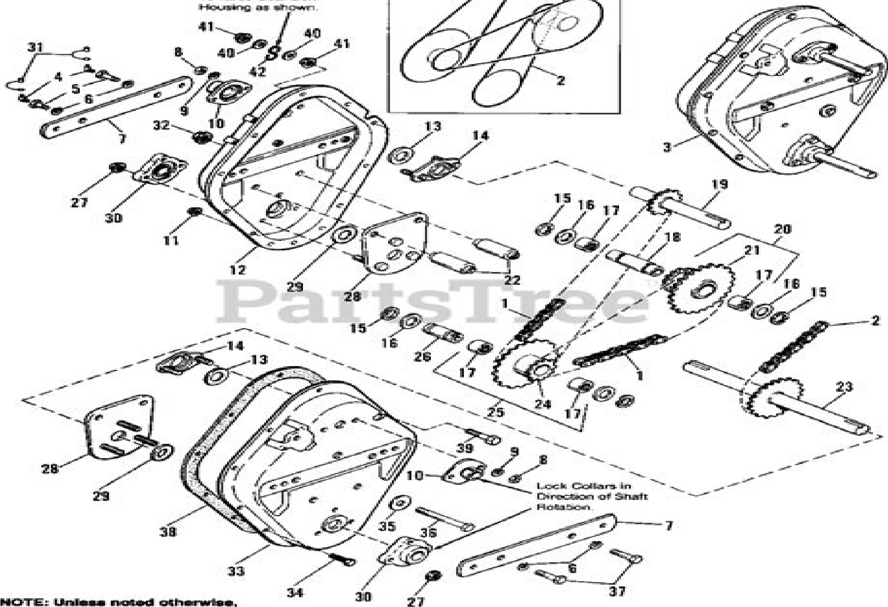
Chain Layout
