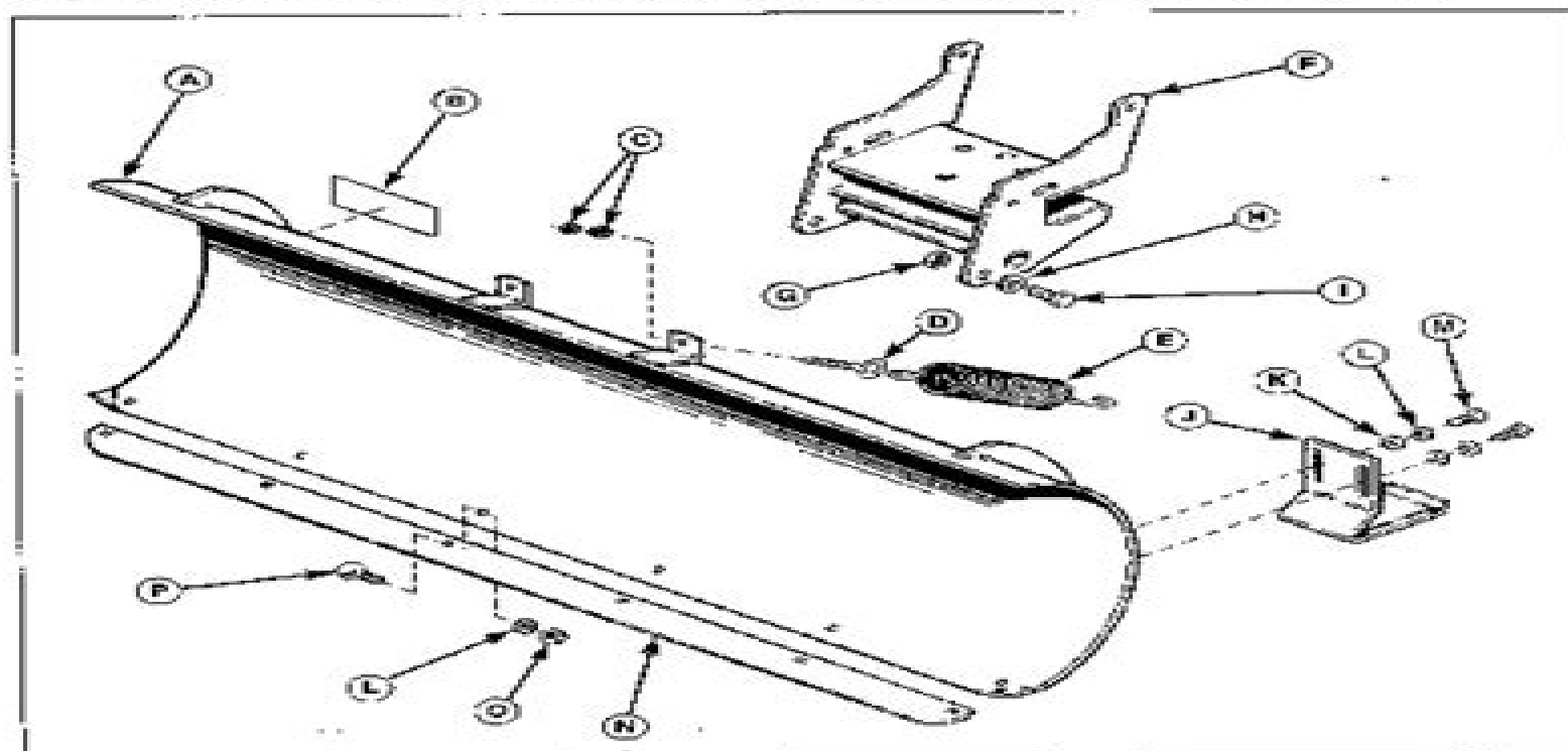
Figure 1. Mfg. No. 1691520 Snow/Dozer Blade Assembly
