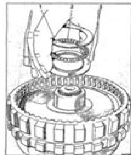
Fig. 71B-16 Fitting the rear and thrust bearing to the outer face of the rear internal gear
