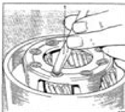
Fig. 71B-14 Staking a pinion pin 1. Oil
